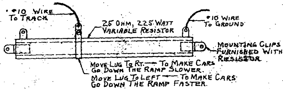
RESISTOR ILLUSTRATION
